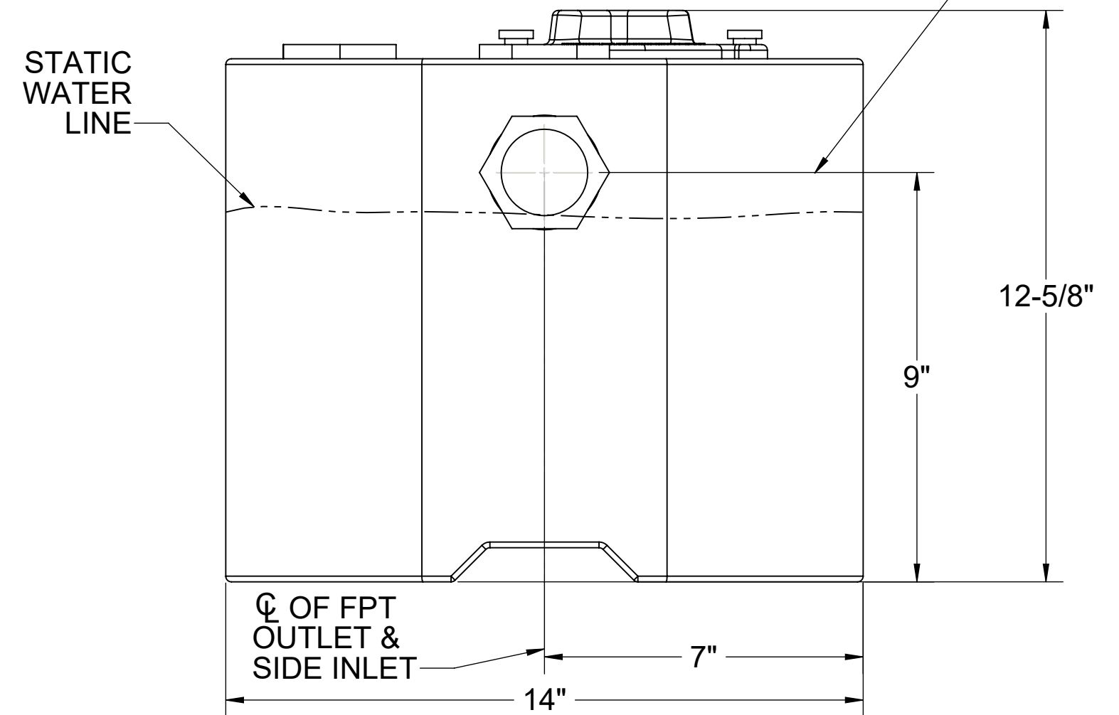
INLET SIDE VIEW
