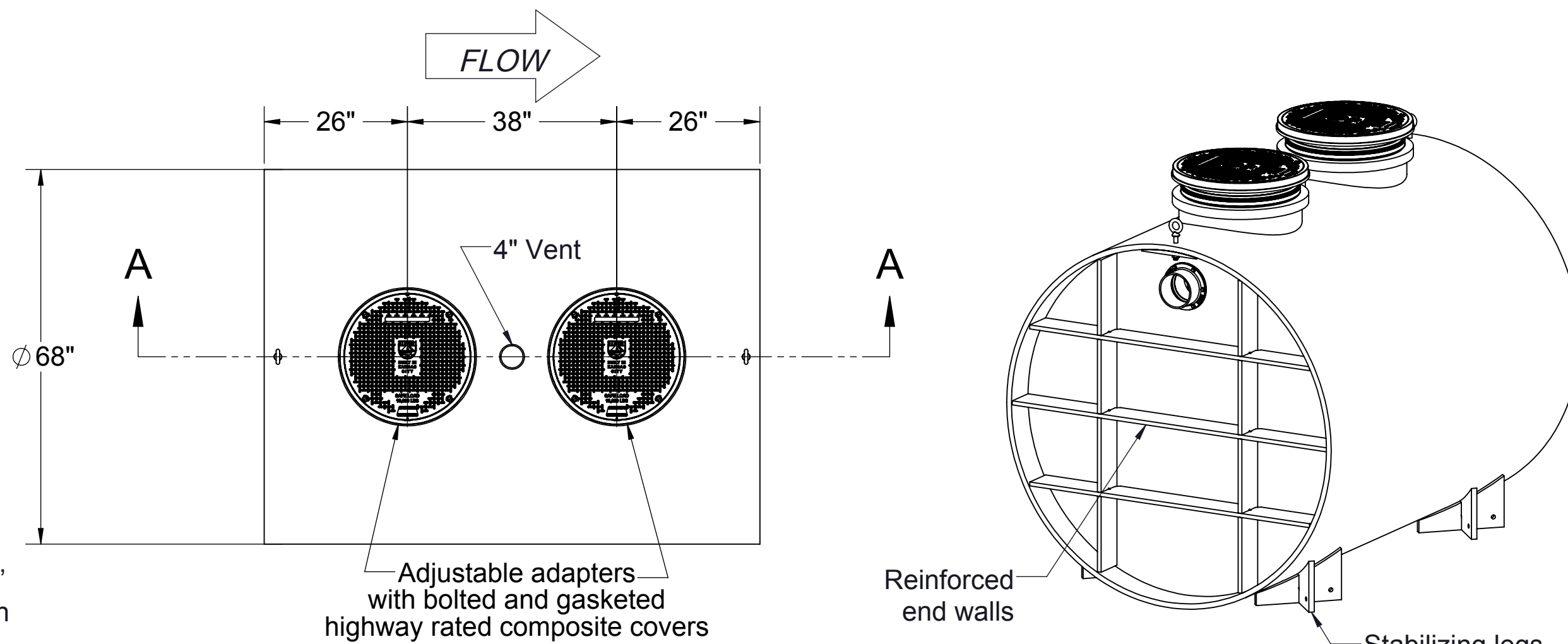
TOP VIEW
